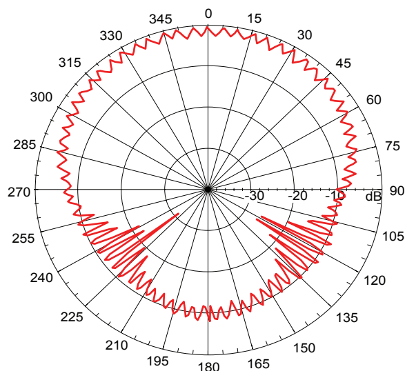
865 MHz
